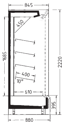
Methos 64.A4 L
